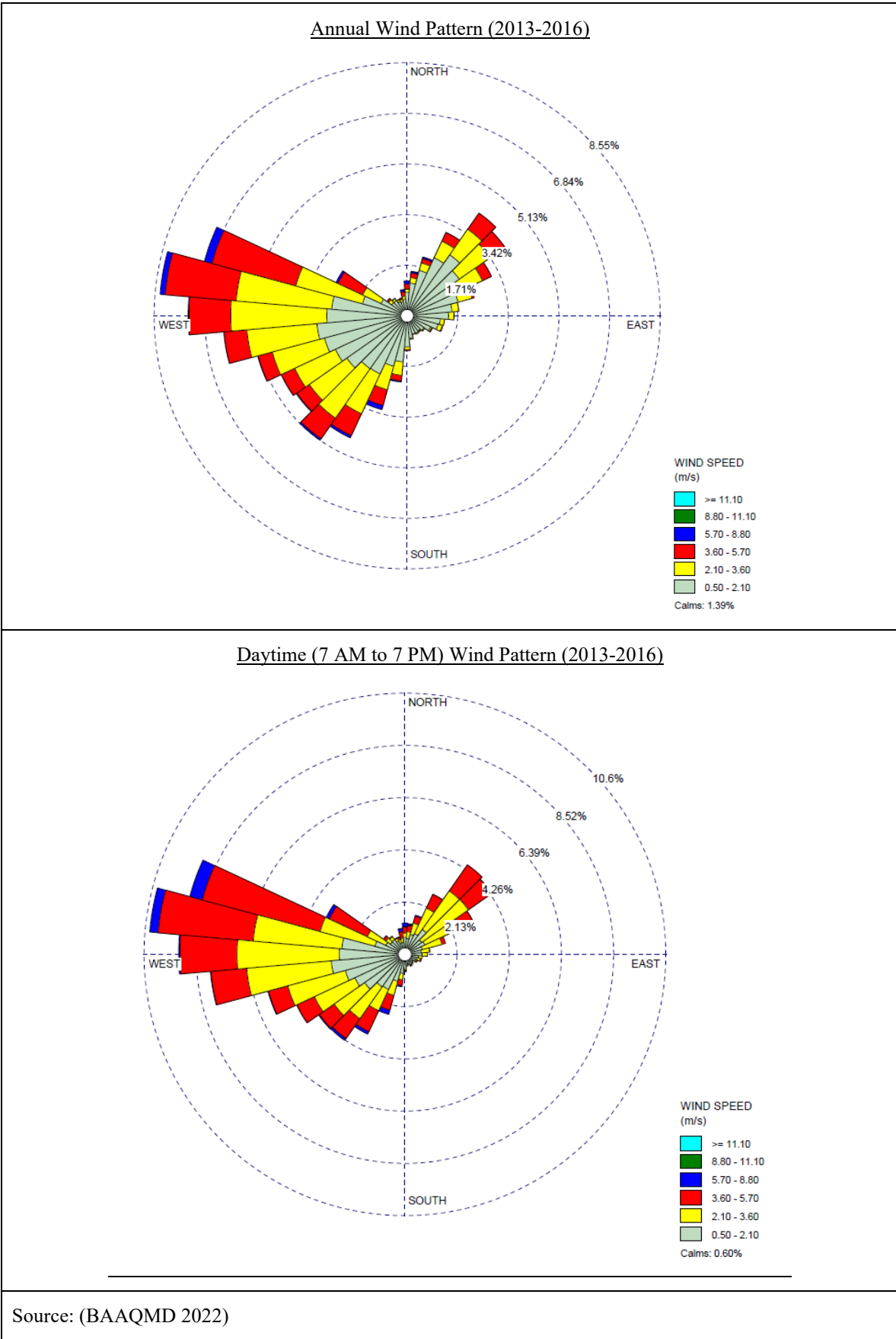
Figure 6-1 Prevailing wind at Livermore Rincon Meteorological Station Carnegie SVRA Resource Management Area Program EIR
